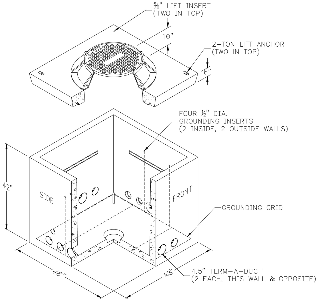
Figure 4— 4' x 4' Manhole Full-Traffic Cover (SI# 7992879)
