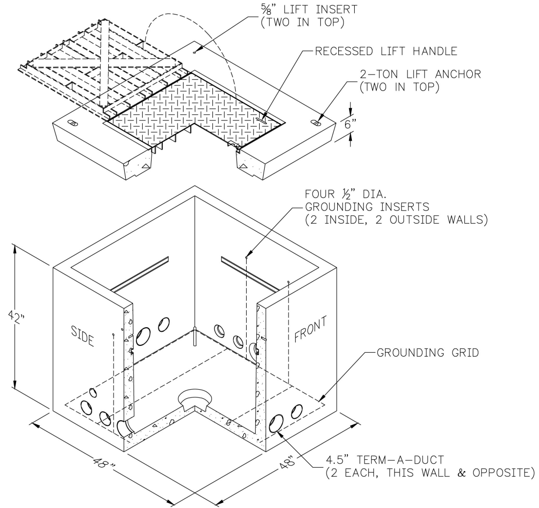
Figure 3— 4' x 4' Manhole Incidental-Traffic Cover (SI# 7992878) (Splice Vault)
