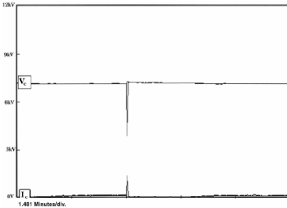
Figure 4 – Typical Voltage and Current Behavior During a Fault
