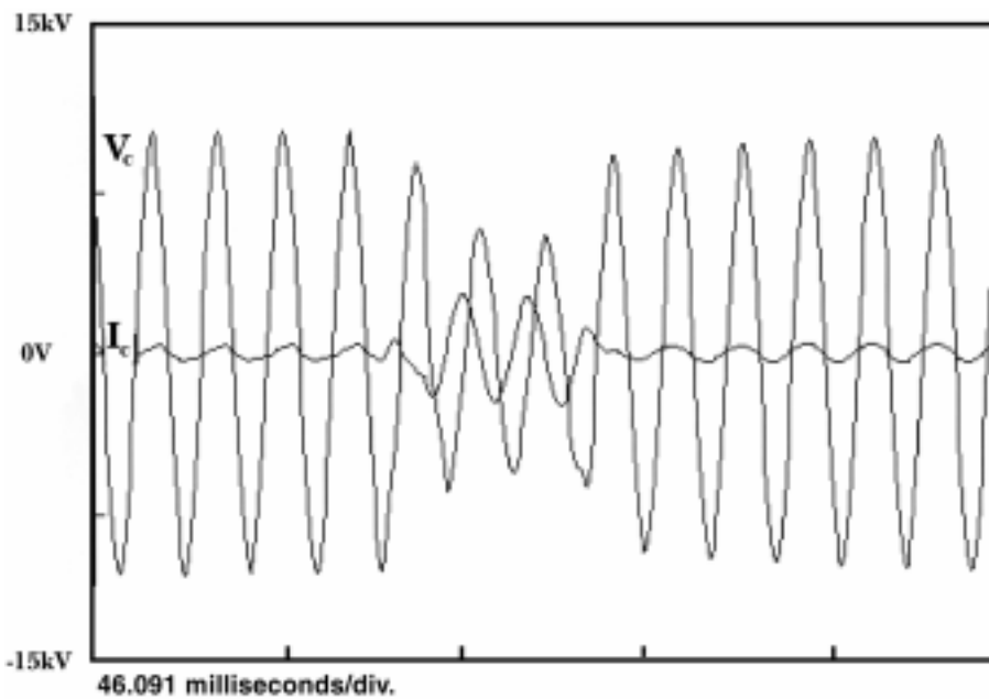
Figure 5 – Typical Voltage and Current Waveforms During a Fault
