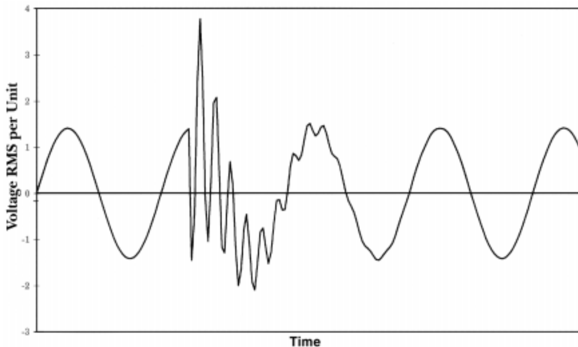
Figure 3 – Typical Capacitor Bank Closing Voltage Waveform
