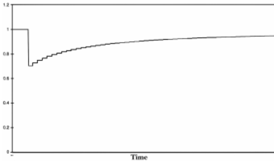
Figure 1 – Typical Motor Start Voltage Profile
