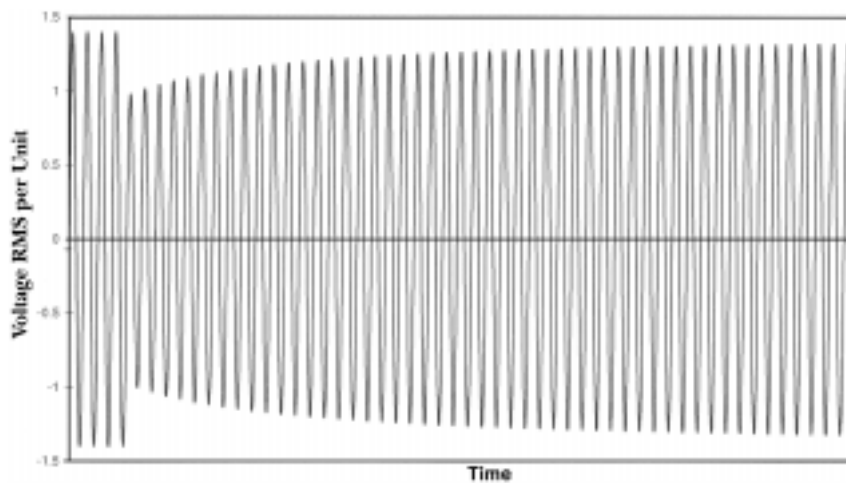
Figure 2 – Typical Motor Start Voltage Waveform
