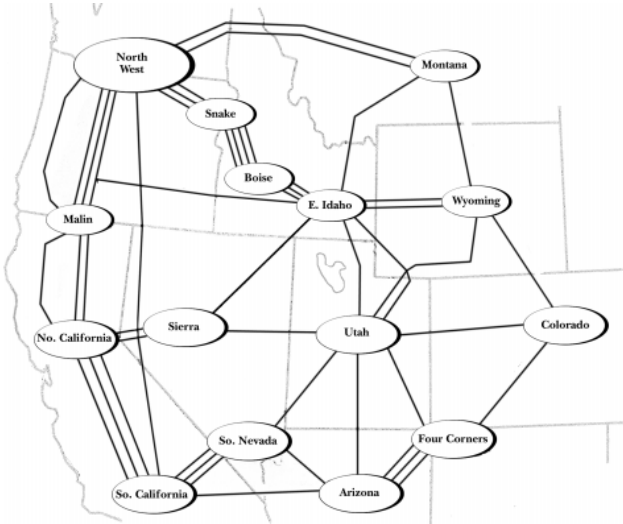
Figure 1 – Simplified Map of Interconnected Western Power System
