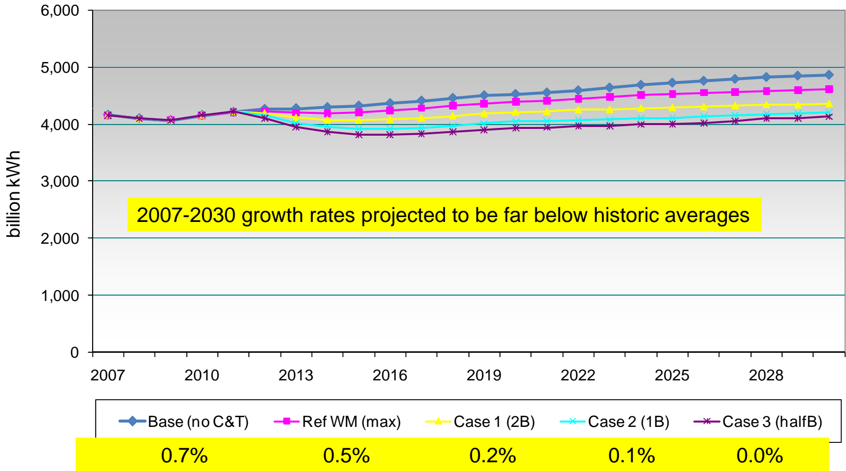
Total Electricity Generation
