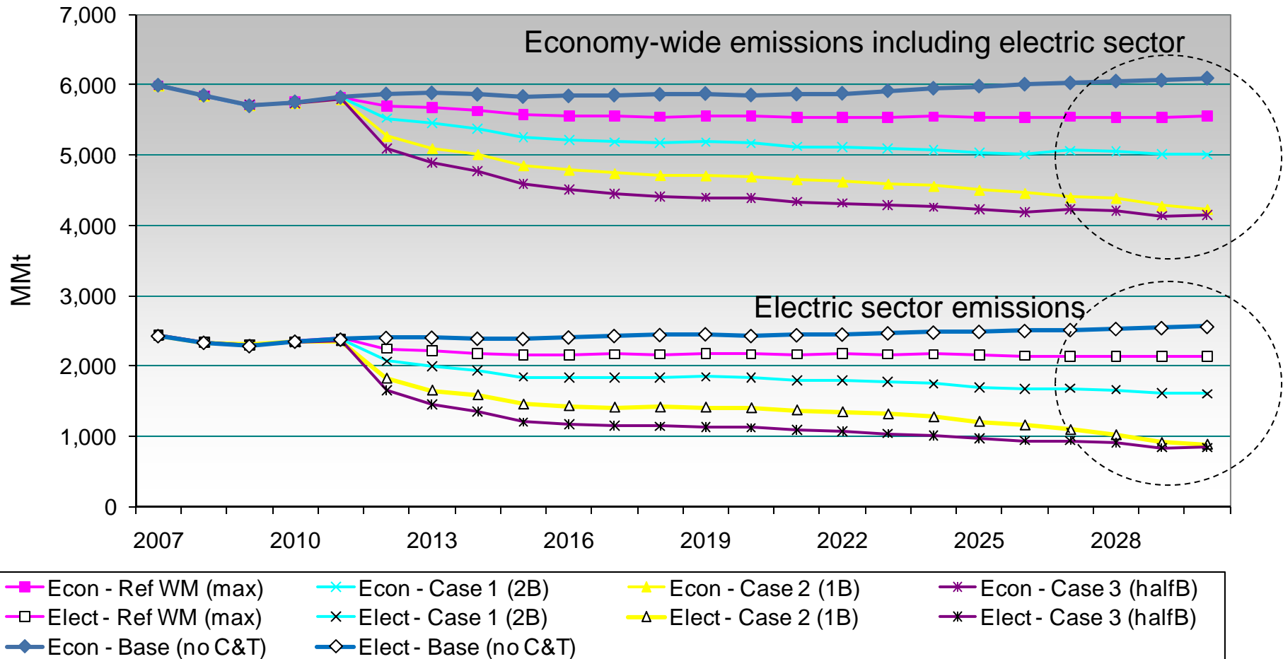
Economy-Wide and Electric Sector CO2 Emissions
