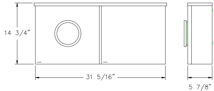
MS252E014 200 Amp Socket Surface mount
