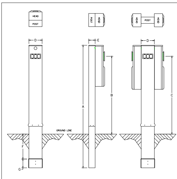
9" X 30" Powerhead
