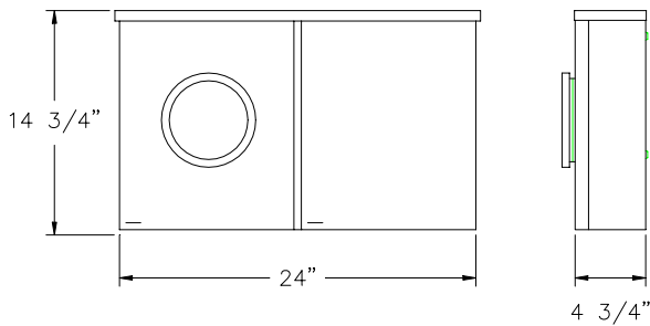
MS462E014 125 Amp Socket Surface mount
