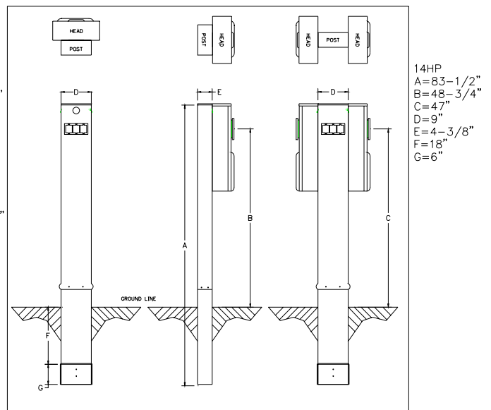
14" X 26" Powerhead
