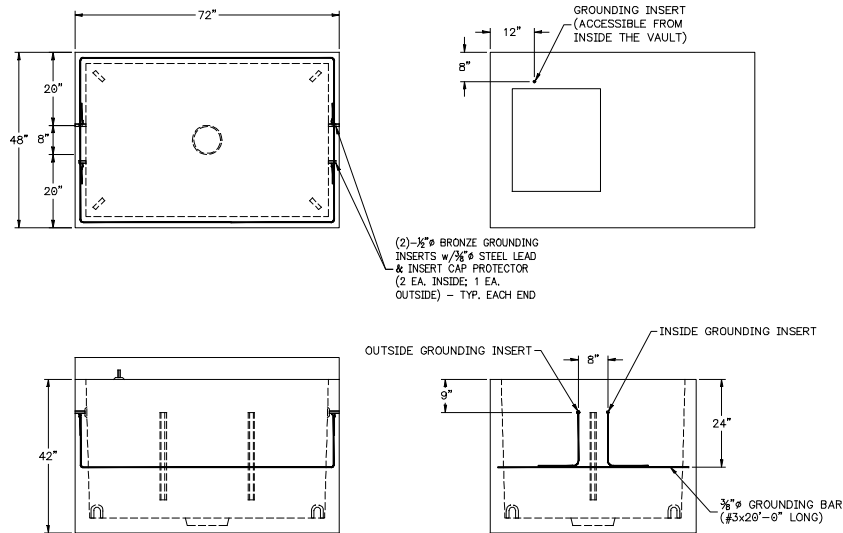
Figure 6—4' x 6' Padvault, Ground Grid Layout
