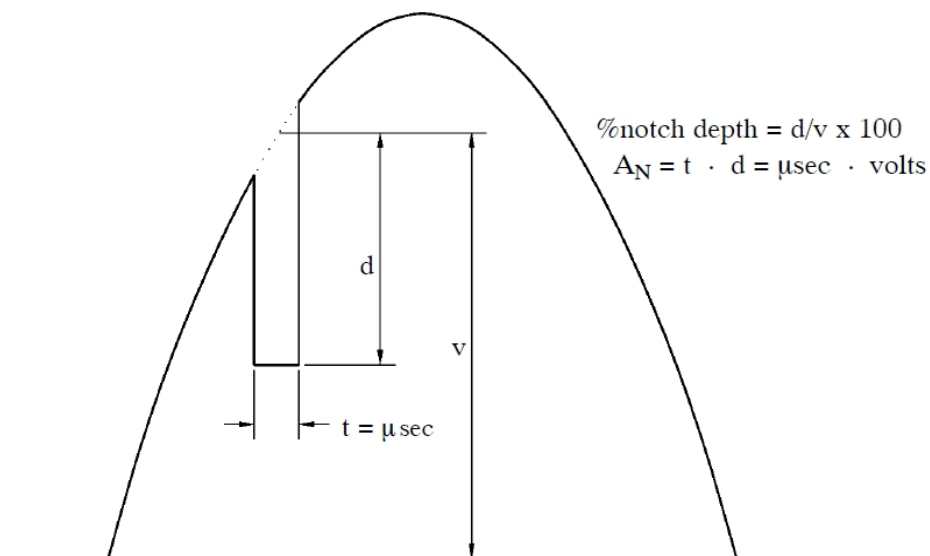
Figure 1—Definition of Notch Depth and Notch Area
